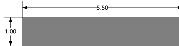
3 HARDIETRIM 5/4 – 5.50" SECTION 5TM1 SCALE = 1/2 : 1
