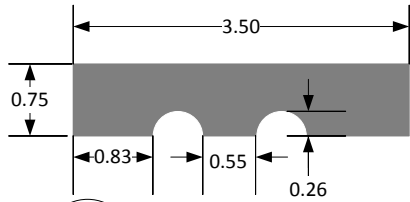
2 HARDIETRIM NT3 4/4 - 3.50" SECTION 4NT31 SCALE = 1/2 : 1
