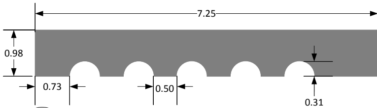
4 HARDIETRIM NT3 5/4 - 7.25" SECTION 5NT31 SCALE = 1/2 : 1
