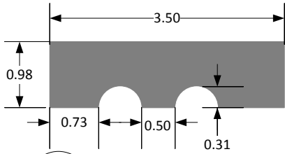
2 HARDIETRIM NT3 5/4 - 3.50" SECTION 5NT31 SCALE = 1/2 : 1
