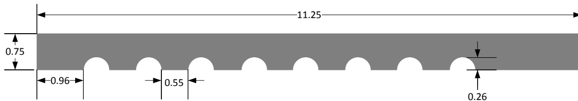
5 HARDIETRIM NT3 4/4 - 11.25" SECTION 4NT31 SCALE = 1/2 : 1
