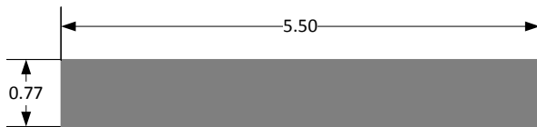
4 HARDIETRIM 4/4 - 5.50" SECTION 4TM1 SCALE = 1/2 : 1
