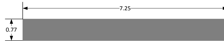
5 HARDIETRIM 4/4 - 7.25" SECTION 4TM1 SCALE = 1/2 : 1
