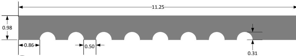
5 HARDIETRIM NT3 5/4 - 11.25" SECTION 5NT31 SCALE = 1/2 : 1
