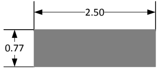
2 HARDIETRIM BATTENS – SECTION BTM1 SCALE = 1/2 : 1
