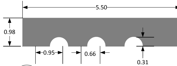
3 HARDIETRIM NT3 5/4 - 5.50" SECTION 5NT31 SCALE = 1/2 : 1
