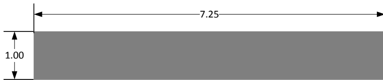
4 HARDIETRIM 5/4 – 7.25" SECTION 5TM1 SCALE = 1/2 : 1
