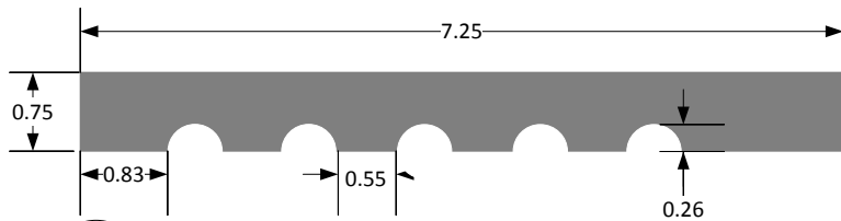
4 HARDIETRIM NT3 4/4 - 7.25" SECTION 4NT31 SCALE = 1/2 : 1
