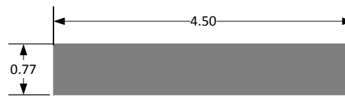
3 HARDIETRIM 4/4 - 4.50" SECTION 4TM1 SCALE = 1/2 : 1
