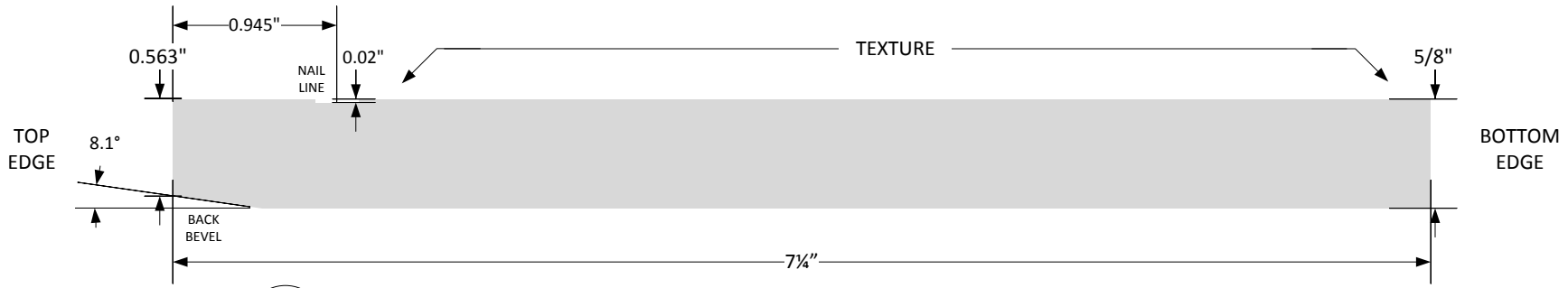
A ALP2 HARDIEPLANK 7 1/4" - SECTION SCALE = 1 : 1
