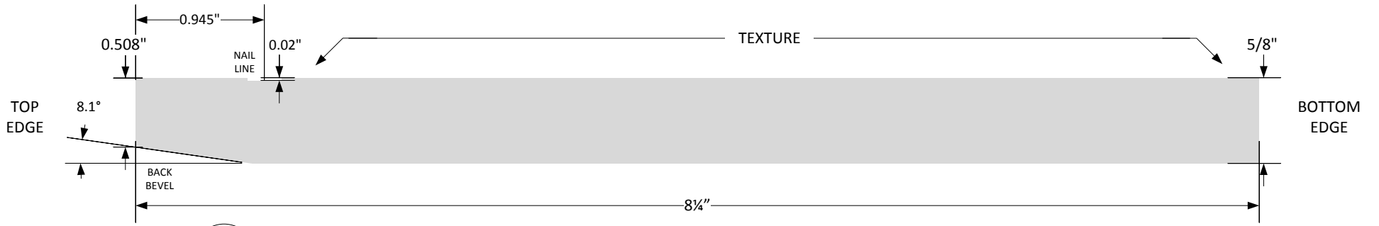
A HARDIEPLANK 8 1/4" - SECTION ALP3 SCALE = 1 : 1
