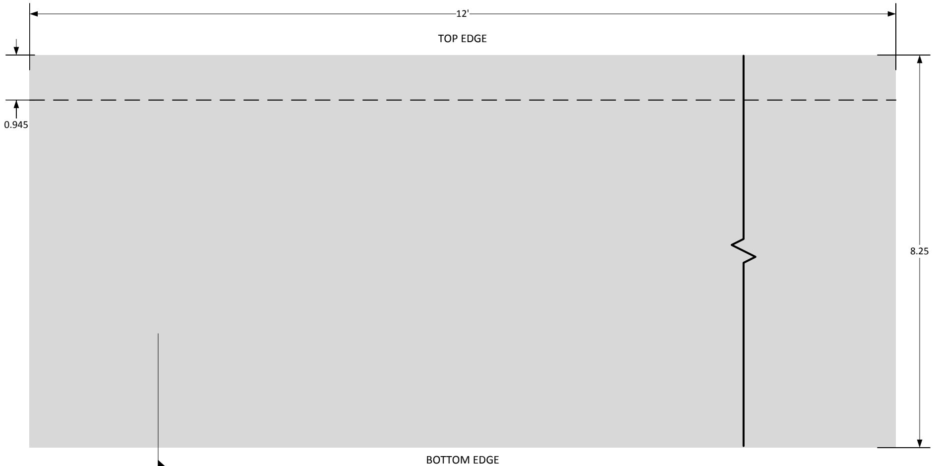
1 ARTISAN LAP SIDING 8 1/4" WIDTH ALP3 SCALE = 1/2 : 1
