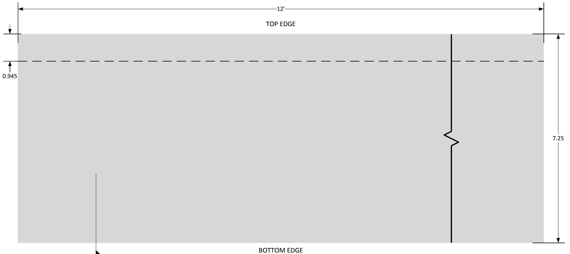
1 ALP2 ARTISAN LAP SIDING 7 1/4" WIDTH SCALE = 1/2 : 1
