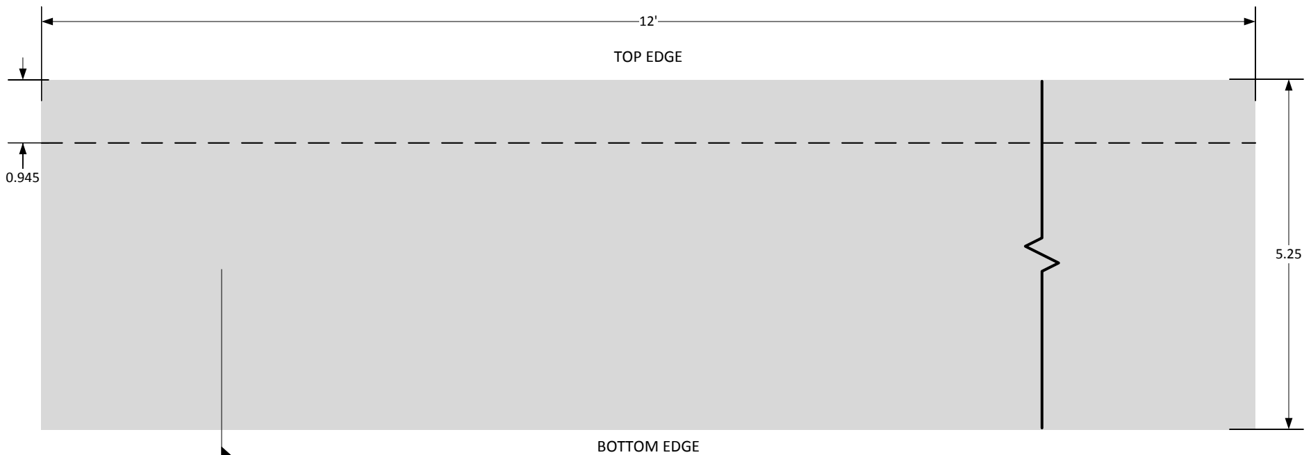
1 ARTISAN LAP SIDING - 5 1/4" WIDTH ALP1 SCALE = 1/2 : 1
