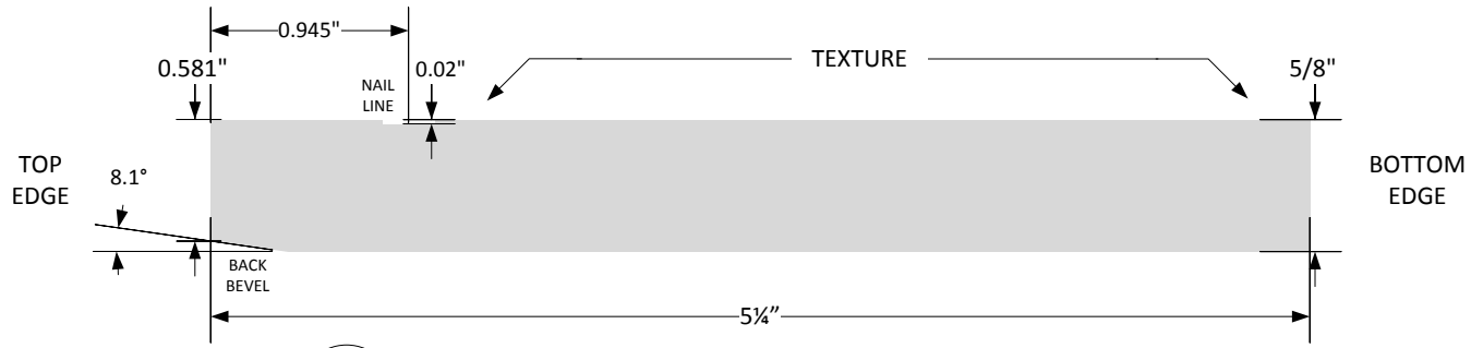
A HARDIEPLANK 5 1/4" - SECTION ALP1 SCALE = 1 : 1
