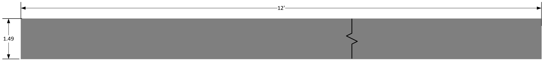
1 ARTISAN TRIM – ALL WIDTHS ATM1 SCALE = 1/2 : 1
