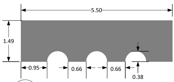
3 ARTISAN TRIM – 5.5" SECTION ATM1 SCALE = 1/2 : 1
