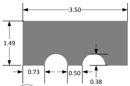
2 ARTISAN TRIM – 3.50" SECTION ATM1 SCALE = 1/2 : 1
