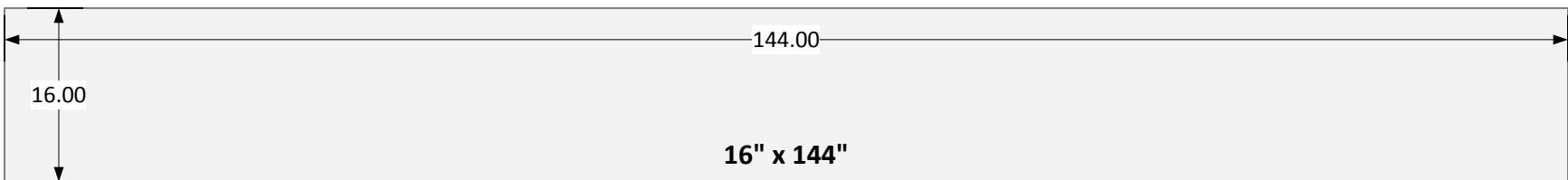
1 NV1 NON-VENTED SMOOTH OR CEDARMILL HARDIESOFFIT PANEL SCALE = 1/16 : 1
