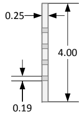
A PANEL SECTION V1 SCALE = 1/4 : 1
