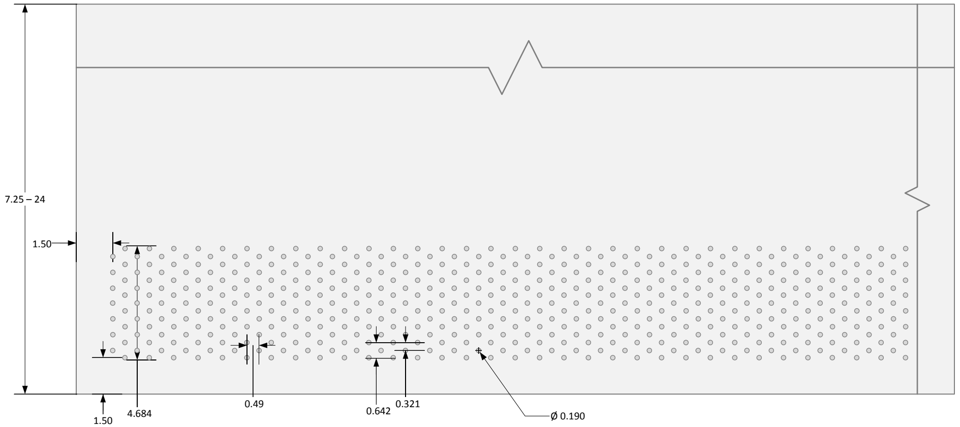
2 VENTED SMOOTH OR CEDARMILL HARDIESOFFIT PANEL V1 SCALE = 1/4 : 1
