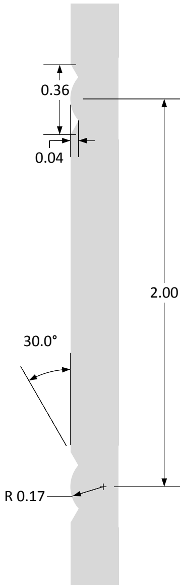
A BP1 EMBOSSING DETAIL
